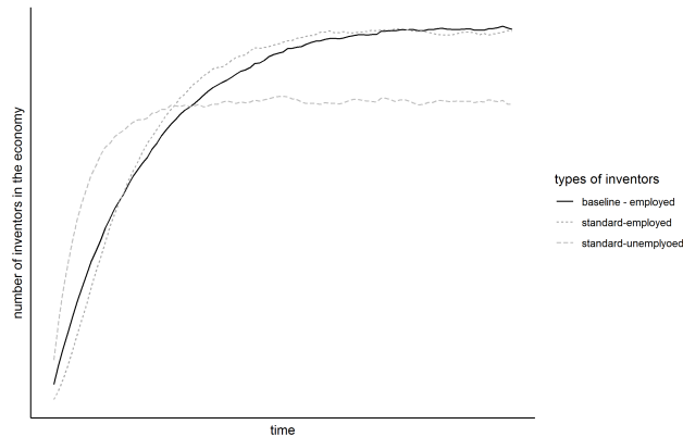
Figure 8: Simulated Example Labor Market with Vacancies
